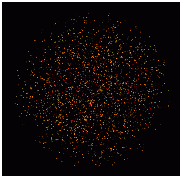
Figure 4 - K stars within 100 light-years
